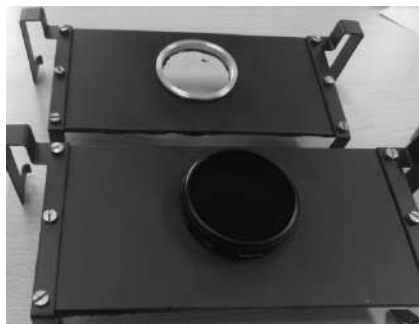
Fig. 6 Protective cover with off/on grey filters Source: authors.
