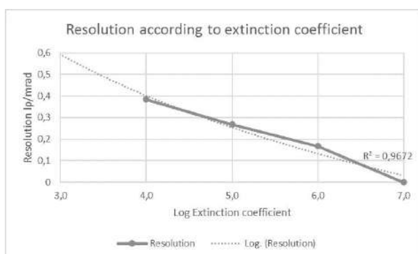
Fig. 8 Graph of the influence of the extinction ratio to the resolution of an imager Source: author.
