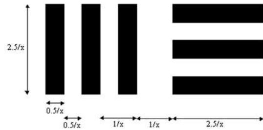
Fig. 3 Dimensions of an element in USAF 1951 test Source: [3].
