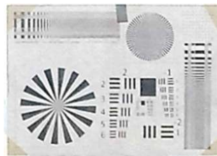
Fig. 7 Captured image from the day branch of the imager Source: authors.
